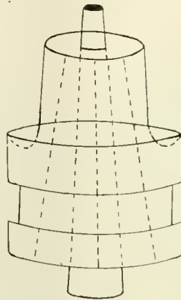
FIG. 1.—EXPANDING AND BEADING TOOL.—ERIE.
